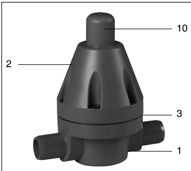
Construction GEMÜ N086, N186
